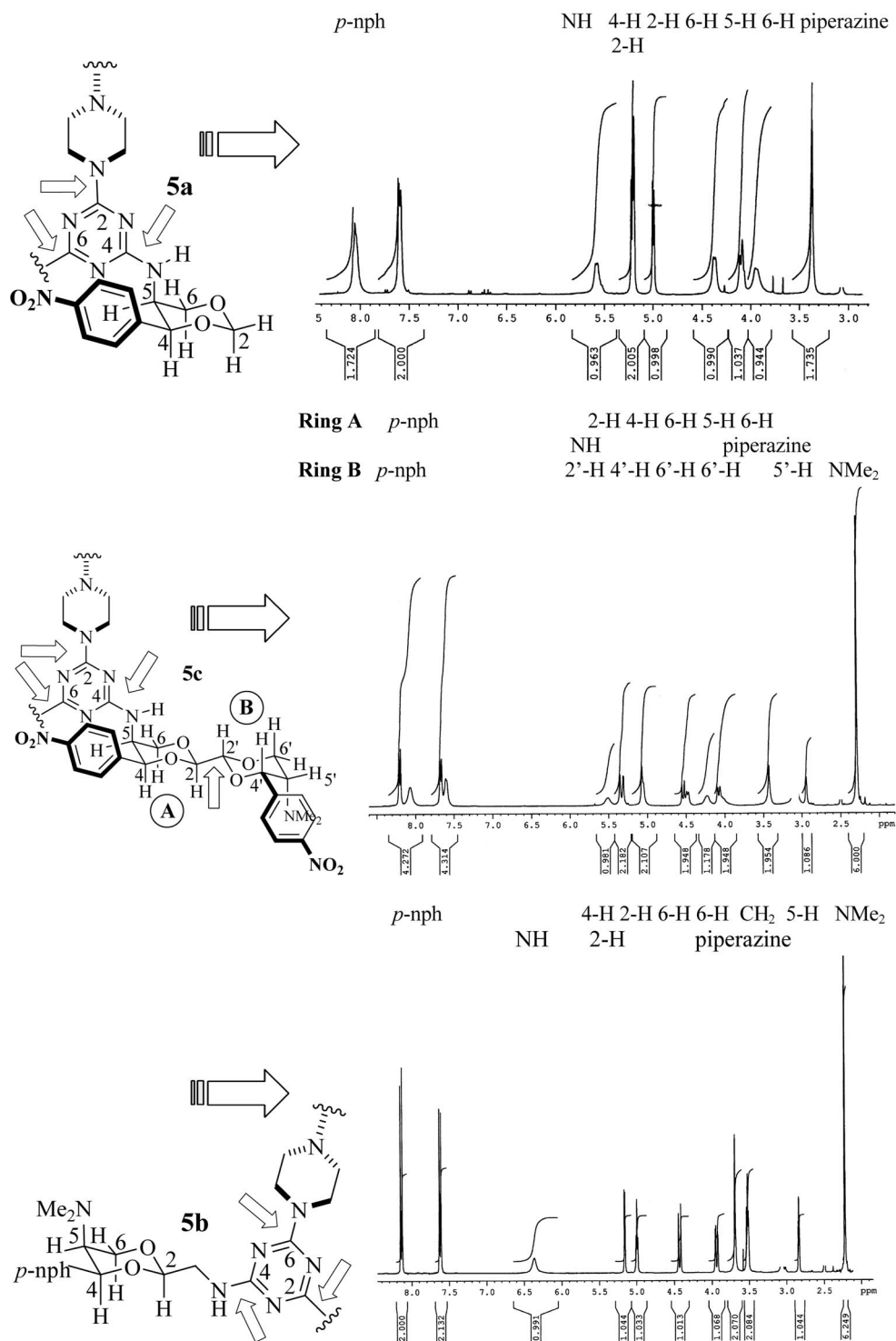
Figure 2. 1 H NMR spectra of compounds 5a–c (353 K, on 400 MHz timescale, [D 6 ]DMSO).
